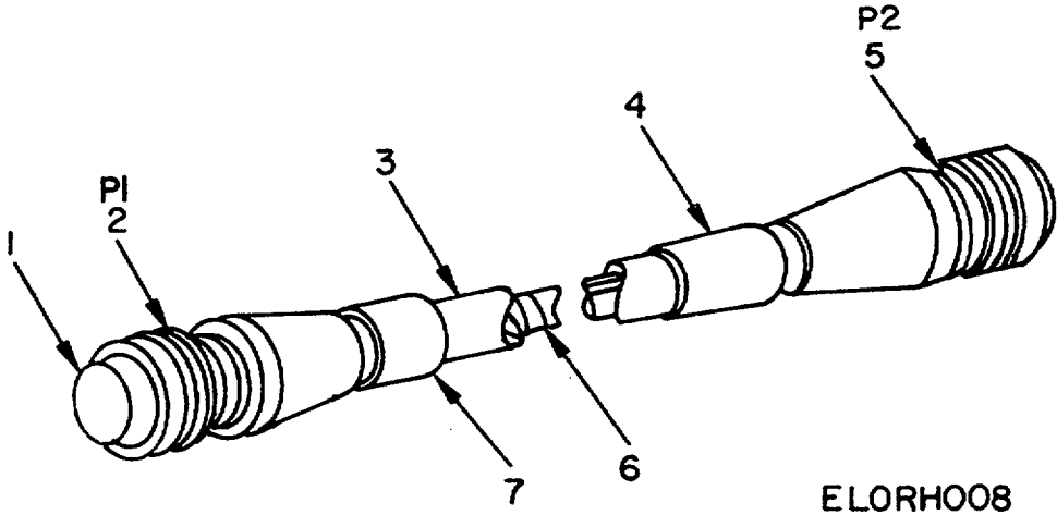
Figure 8. Cable Assembly A02VS309-1.
