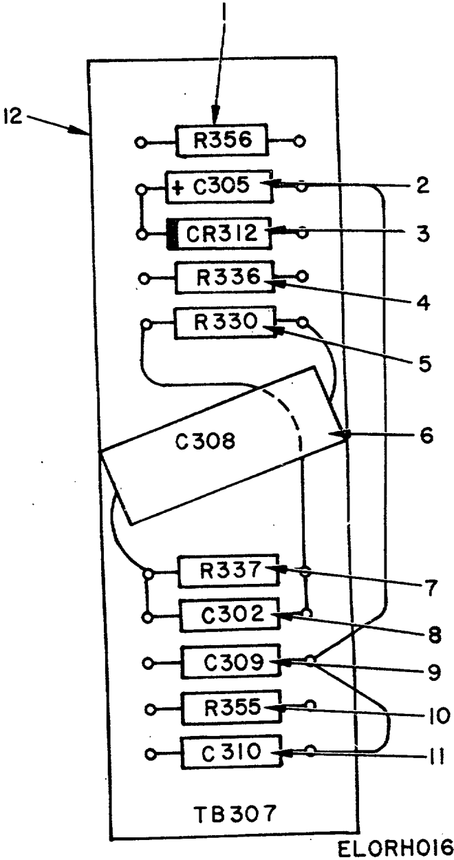
Figure 15. Component Assembly TB 307.
