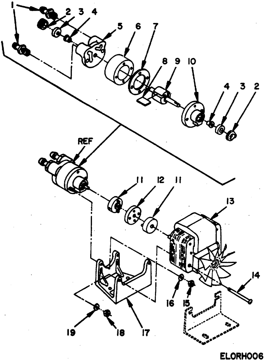
Figure 6. Pump Assembly, Air.
