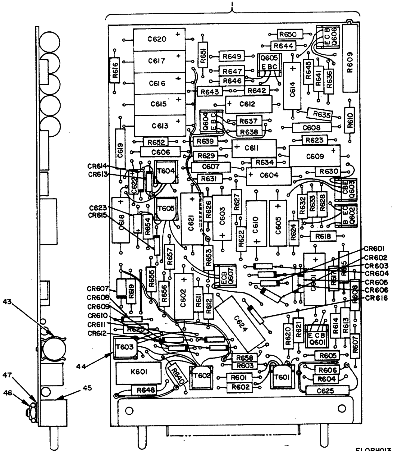
Figure 13. Component Assembly, Actuator-Simulator-Card (Sheet 1 of 2).
