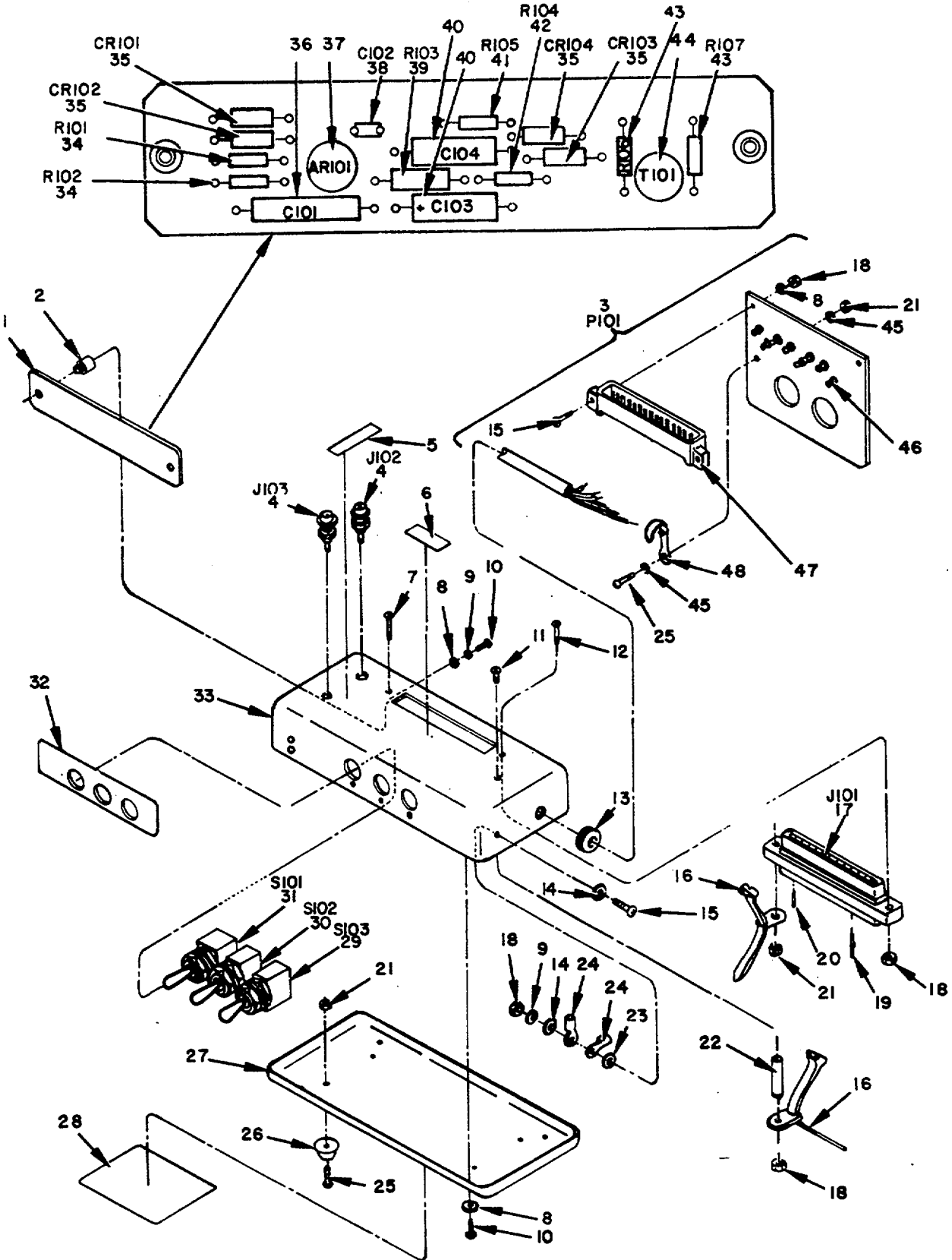
Figure 7. Box Assembly, Adapter.
