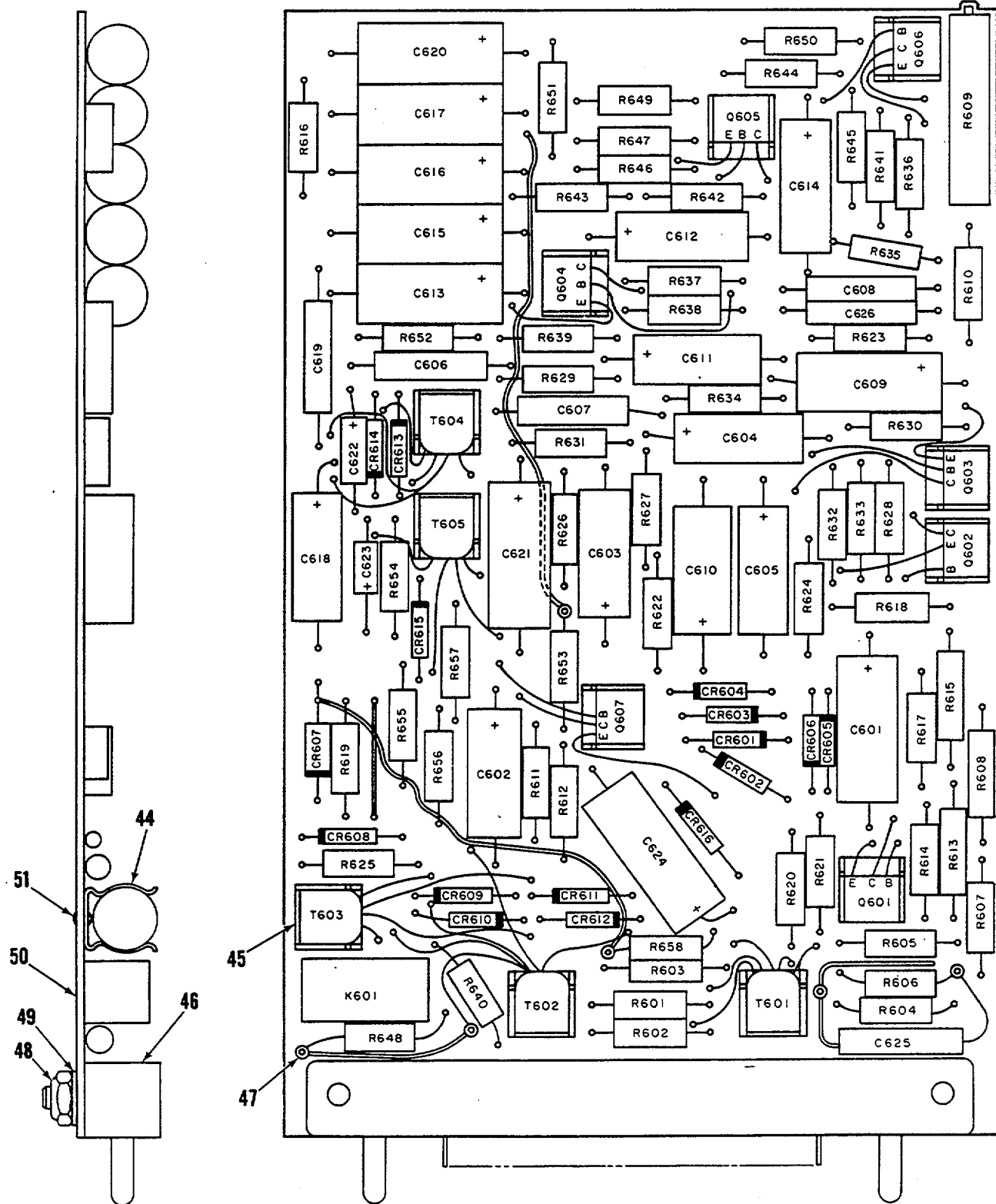
Figure 13A. Component Assembly, Actuator-Simulator-Card A02V3048-3 (Sheet 1 of 2).
