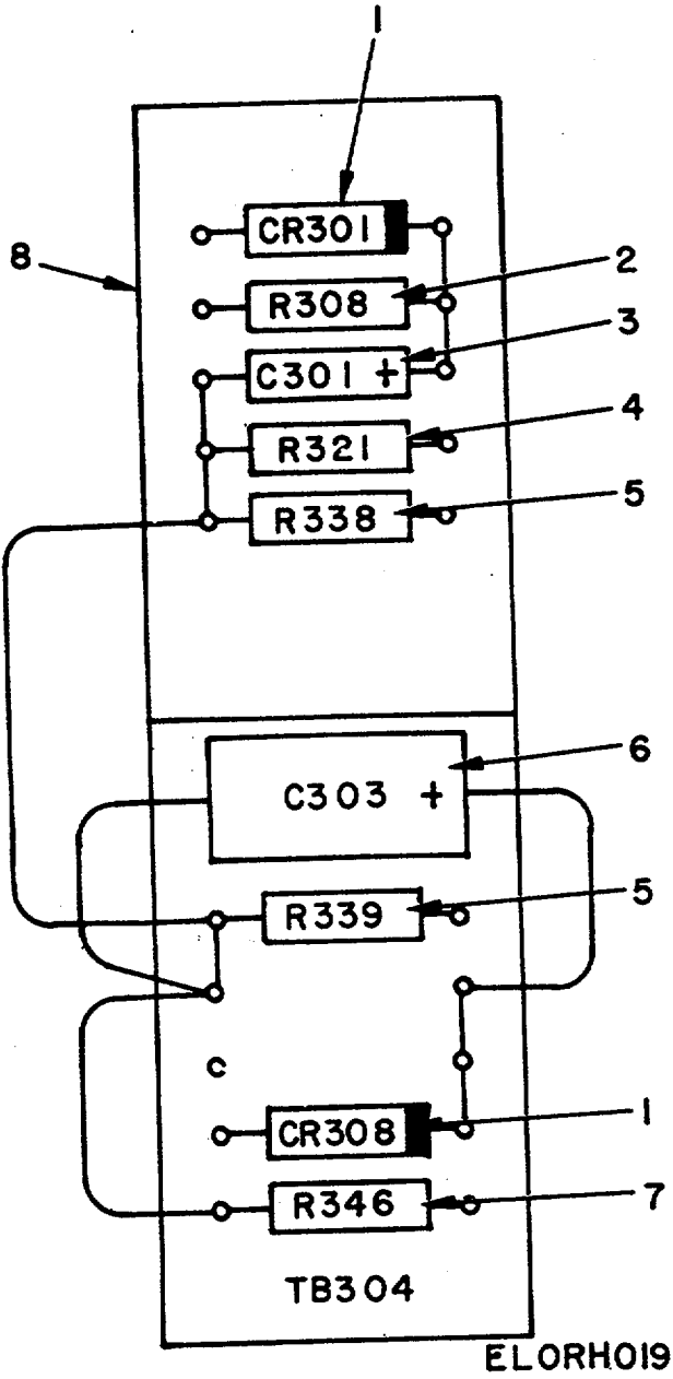
Figure 18. Component Assembly TB 304.
