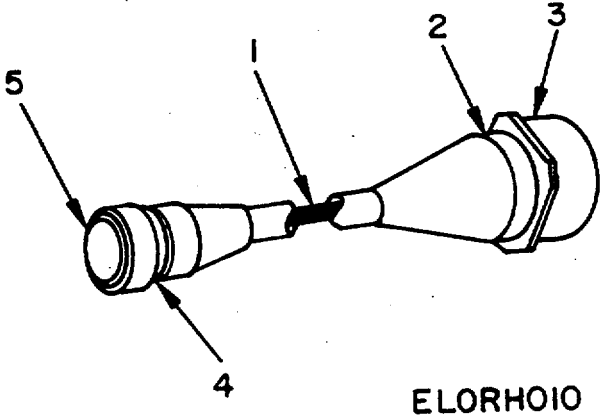
Figure 10. Cable Assembly A02VS309-14.
