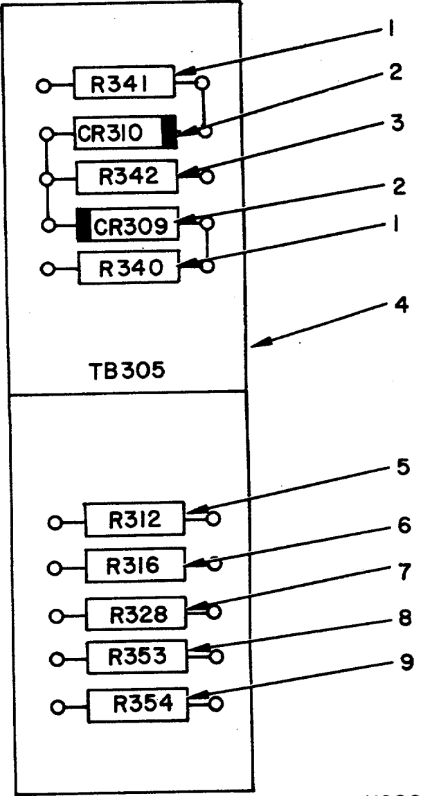
Figure 19. Component Assembly TB 305.
