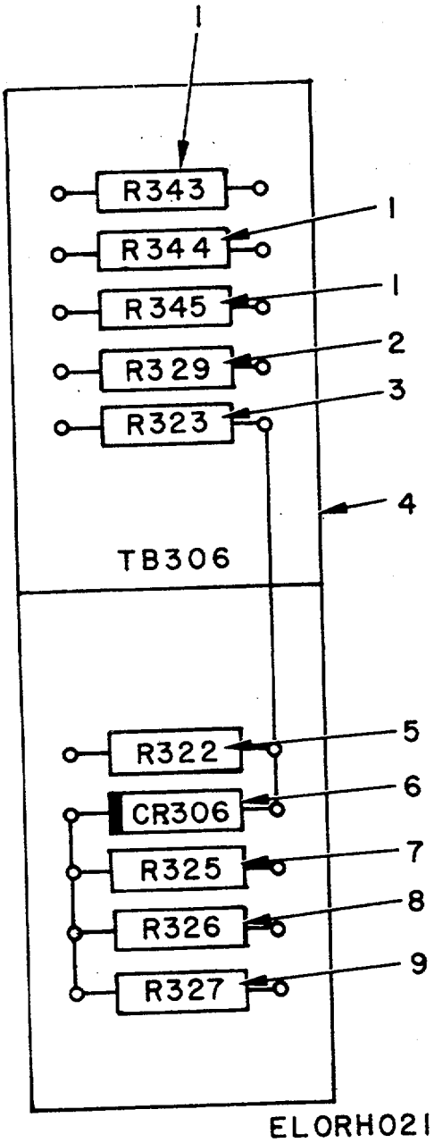
Figure 20. Component Assembly TB 306.
