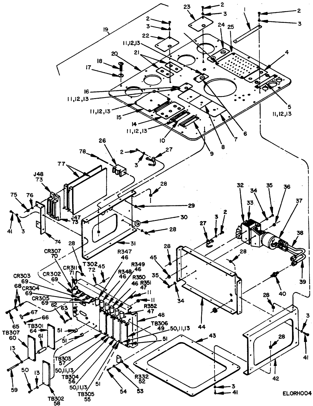
Figure 4. Test Set, Amplifier AN/ASM-121, Front Panel and Components Location.
