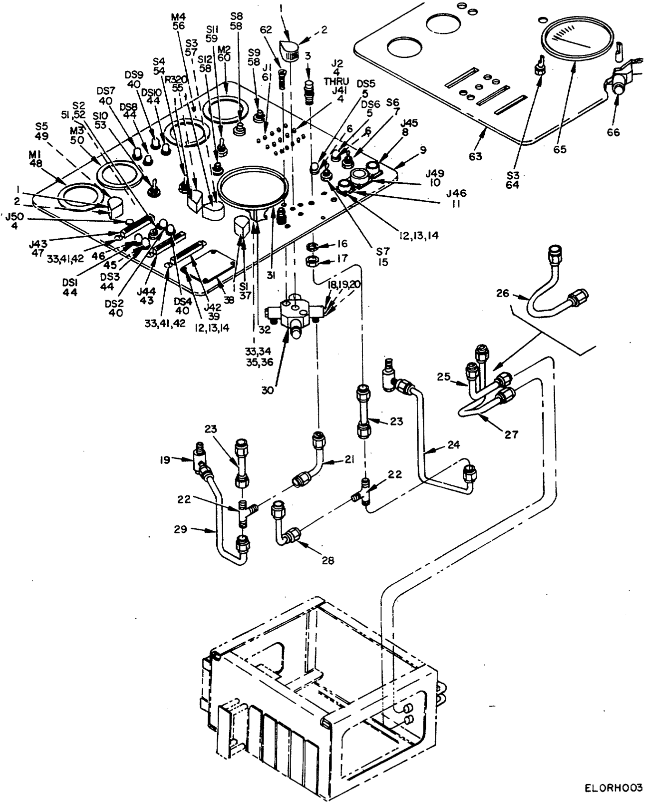
Figure 3. Test Set, Amplifier AN/A,A-121, Panel and Tubes Assemblies.
