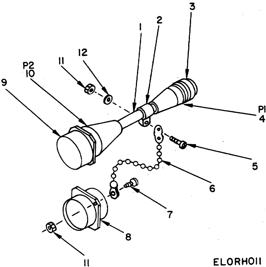
Figure 11. Cable Assembly A02VS309-15.
