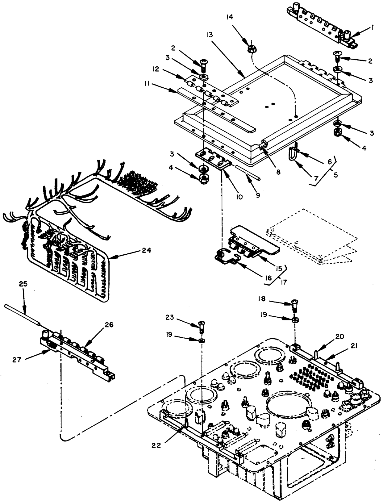
Figure 2. Test Set, Amplifier AN/ASM-121, Frame and Retainer Assemblies.
