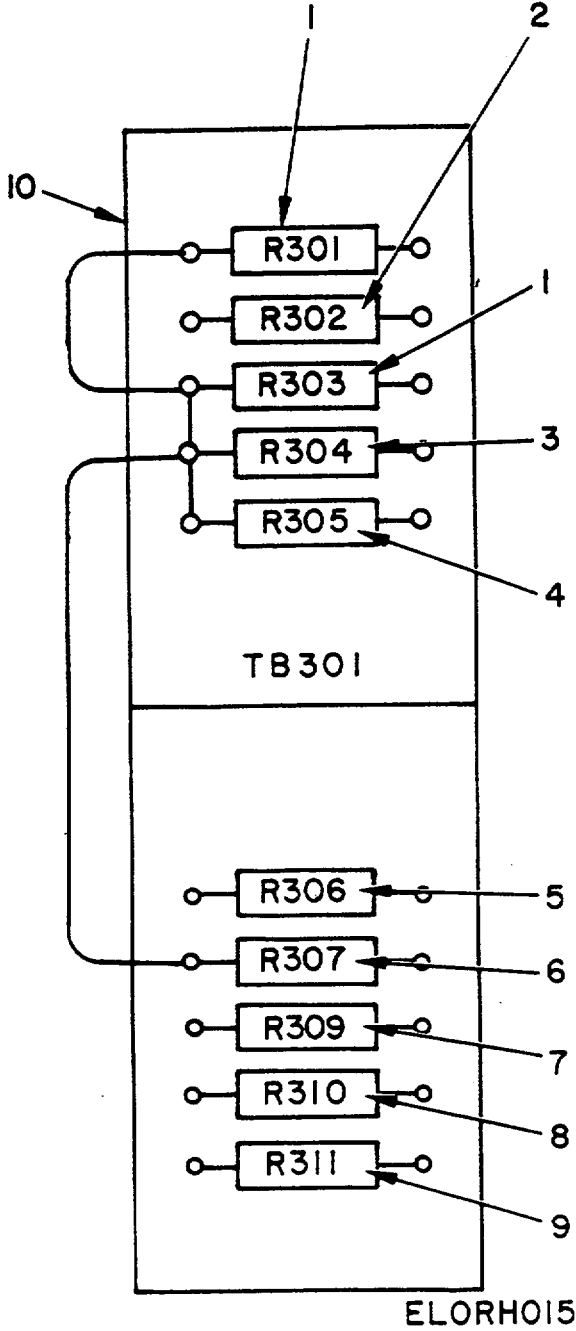
Figure 14. Component Assembly TB 301.
