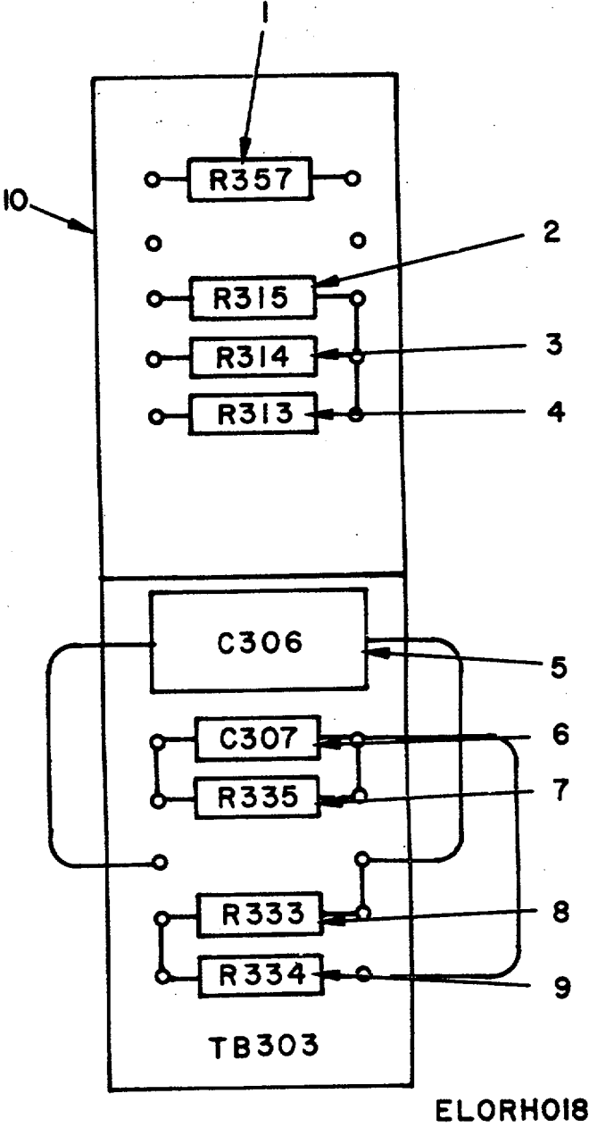
Figure 17. Component Assembly TB 303.
