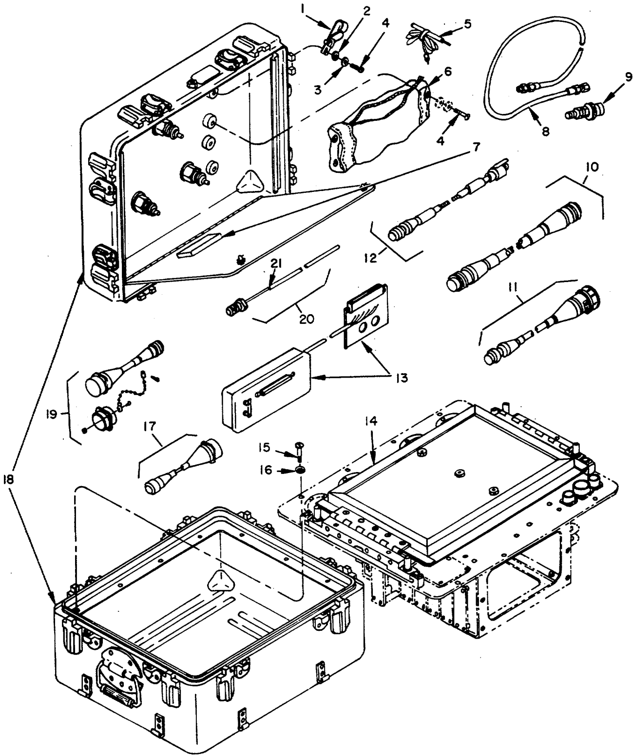
Figure 1. Test Set, Amplifier AN/ASM-121, Case and Cable Assemblies.
