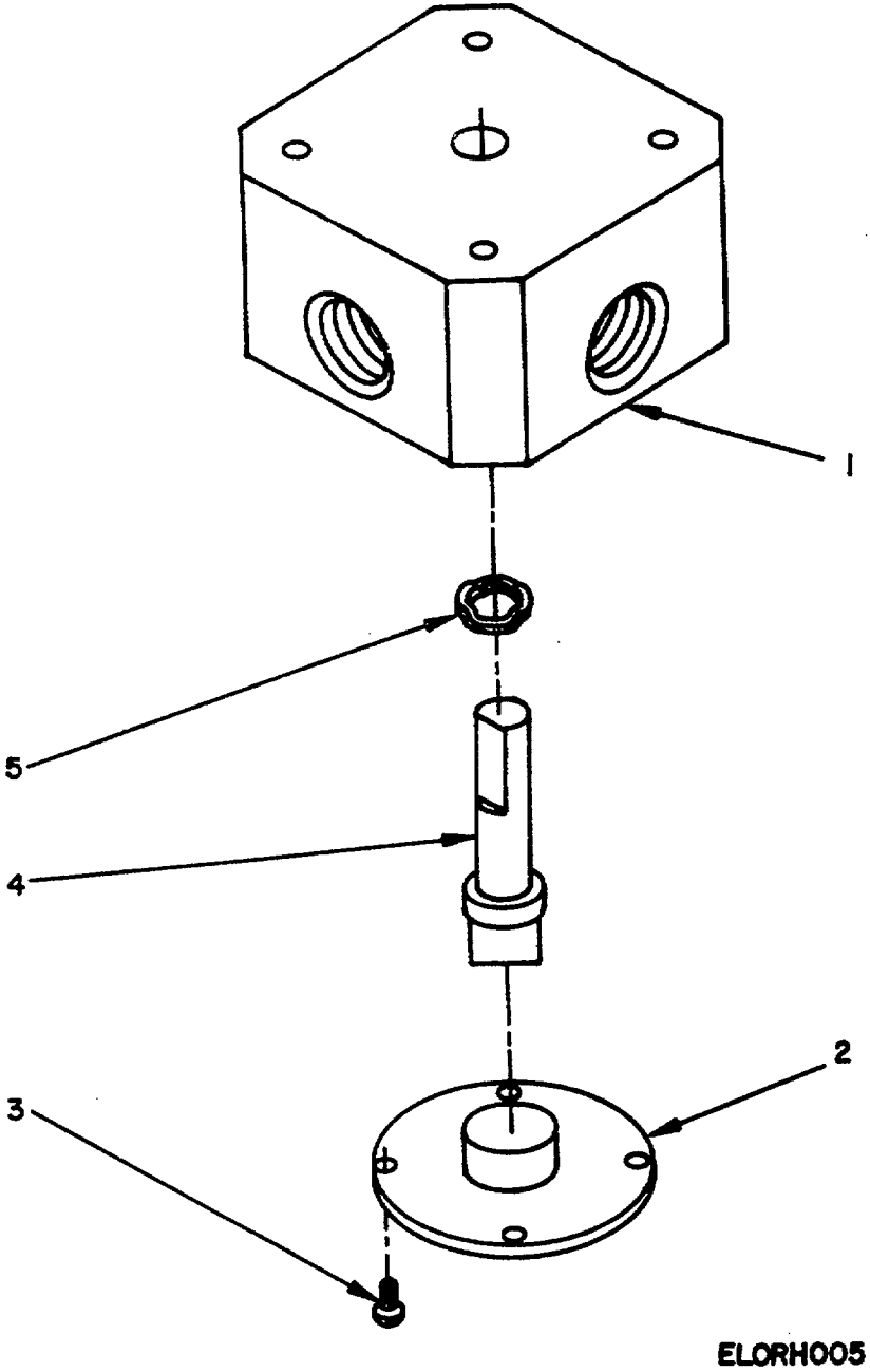
Figure 5. Valve Regulator.
